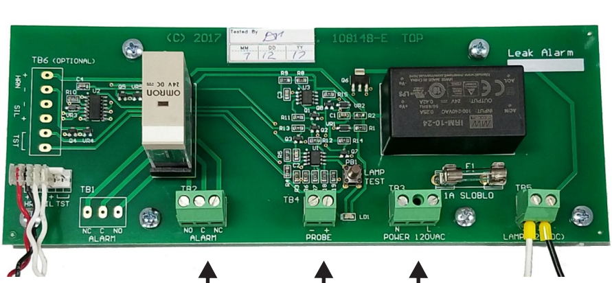
Alarm Contact (optional) Probe AC Power
